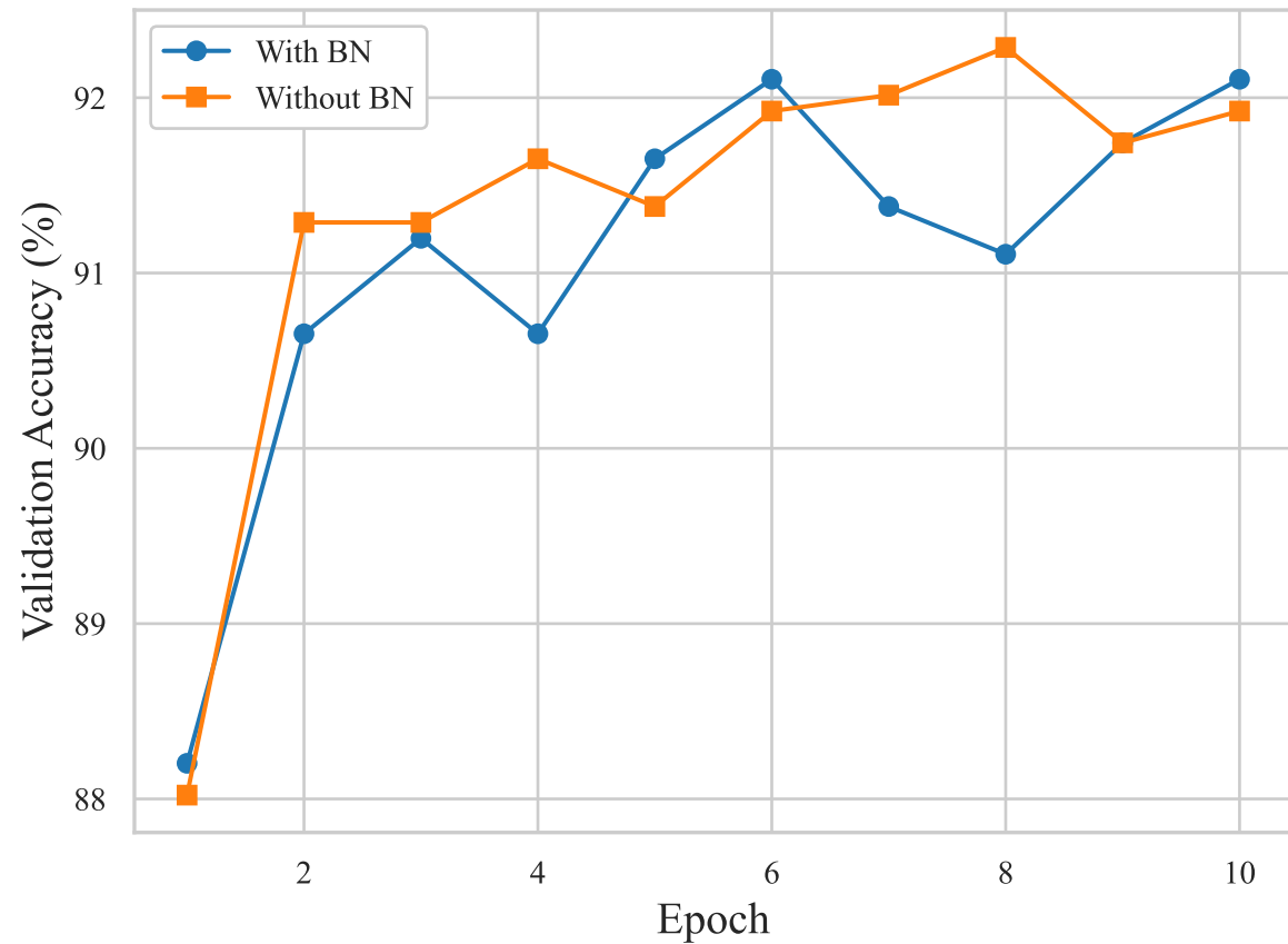
Plot 5: With vs. Without Batch Normalization
